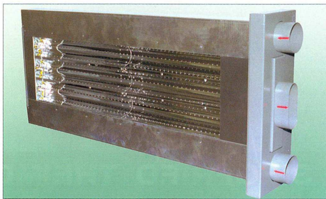
UV-dryer, 1200 mm, 30 kW inmounting unit.
